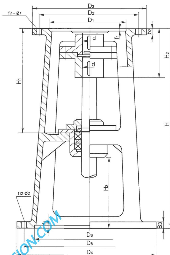
图5-14 JXLD型机架
